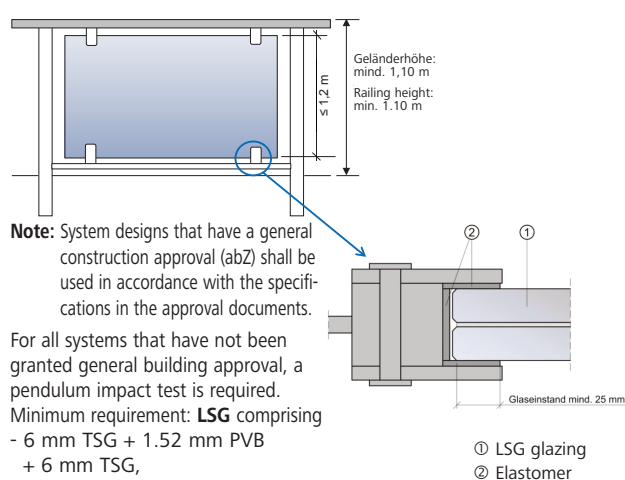
Figure 5: Cross section of edge clamp holder
