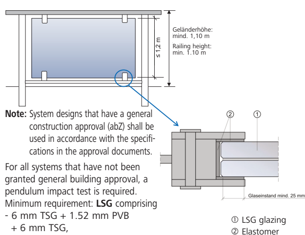
Figure 5: Cross section of edge clamp holder
